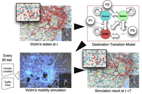
Figure 3: Multi-agent simulator
