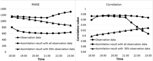
Figure 14. Accuracy with respect to observation data loss
